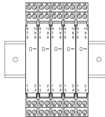
Vertically installation
