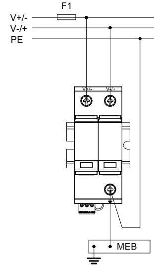
24 V, 48 V, 220 V DC power supply system
