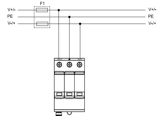
Photovoltaic power system
