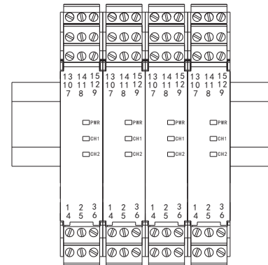
Vertically installation
